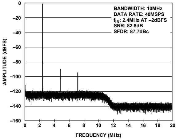
Figure 16. AD9262BCPZ-10 Single-Tone FFT with f_{IN} = 2.4 MHz
