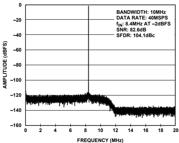
Figure 18. AD9262BCPZ-10 Single-Tone FFT with f_{IN} = 8.4 MHz
