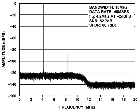
Figure 17. AD9262BCPZ-10 Single-Tone FFT with f_{IN} = 4.2 MHz
